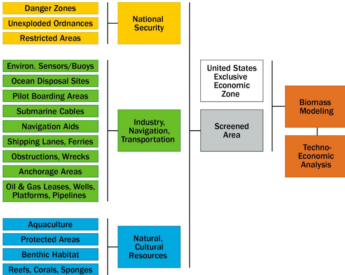
Figure 7.18. General marine area screening methodology based on NOAA's Aquaculture Opportunity Area workflow. Screened areas are merged with G-MACMODS biomass productivity and TEAs.
