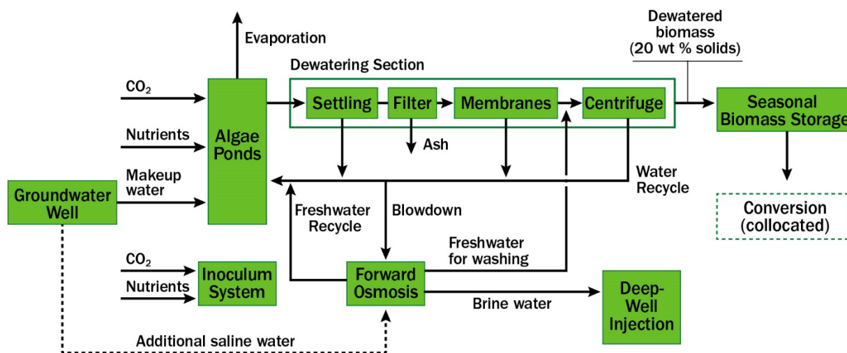
Figure 7.6. Site-level algae farm techno-economic framework used in this study, from cultivation to harvesting and seasonal biomass storage
