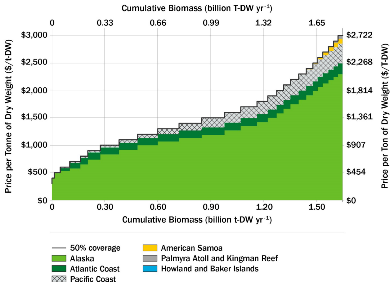
Figure 7.26. Region-specific stepwise cost-supply curve with the representative scenario and 50% area coverage. Note that unlisted regions have costs exceeding $3,000/t-DW.
