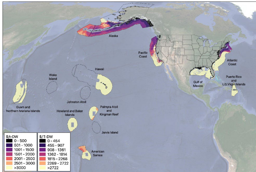
Figure 7.23. U.S. EEZ with screened-inclusive areas and techno-economic results for macroalgae biomass for the representative scenario, with areas > \$3,000/t\text{-DW} ( > \$2,722/T\text{-DW} ) being grouped into a common class
