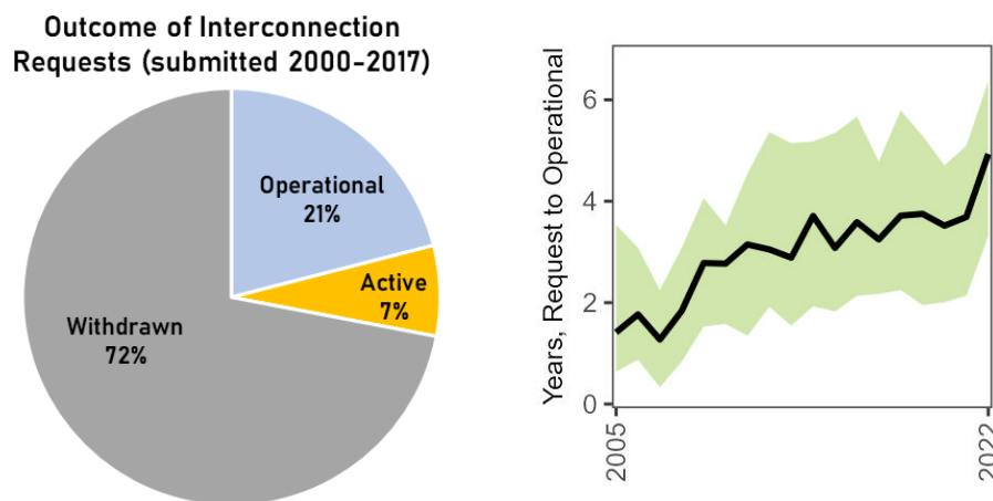
Figure IV-17. Indicators of the challenges facing transmission interconnection, planning, and construction. Right panel shows the median (black line) and interquartile range (green envelope) of years from generator interconnection request to operation for projects dating back to 2005.
