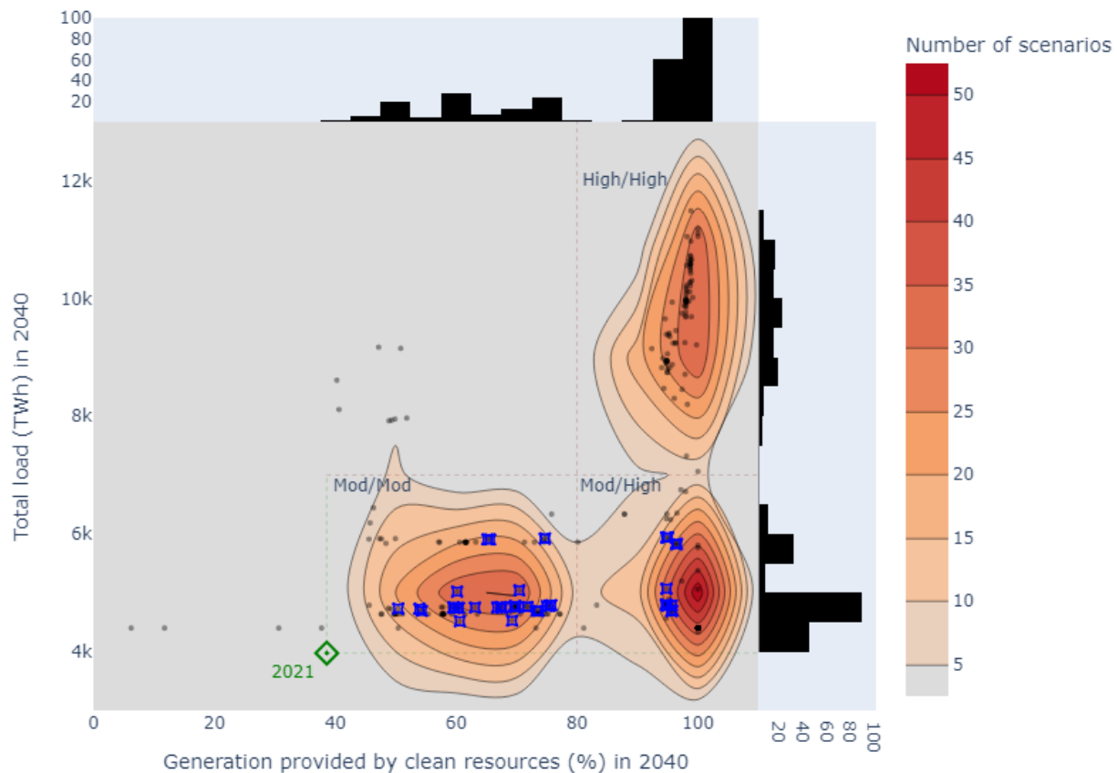
Figure VI-2. Histograms and contour plot for all study scenarios describing the amount of clean energy generation (in percentage of total annual generation) and the total annual load in 2040 with high DER scenarios indicated.
