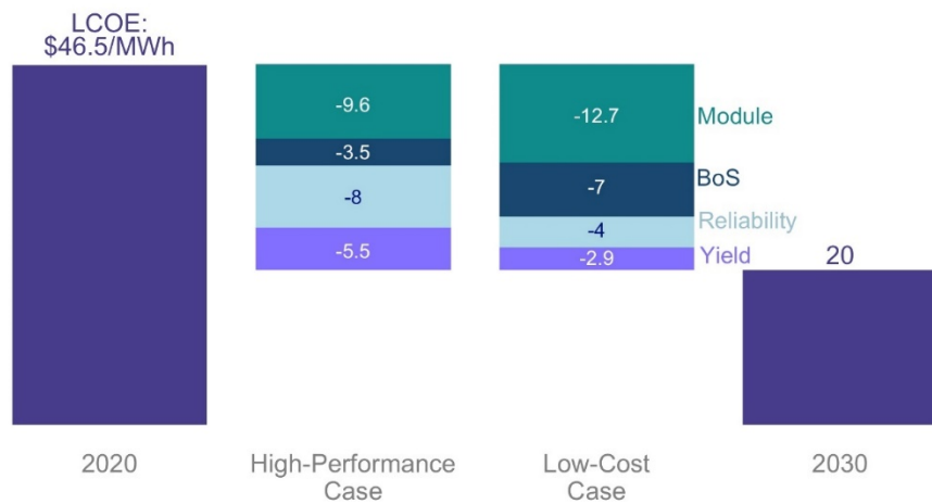
Figure 6 - 5. Two example cases that achieve the 2030 target for utility-scale PV LCOE. Many possible technology trajectories can reach the same cost target.
