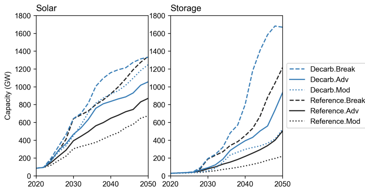
Figure 2-B-2. Solar (left) and storage (right) capacity under a range of cost assumptions
