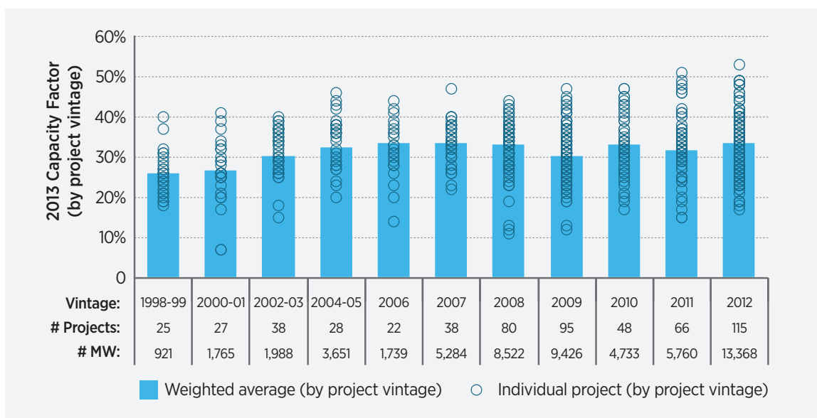
Figure 2-30. Wind project capacity-weighted average capacity factors for 2013 by commercial operation date for project vintages 1998–2012
