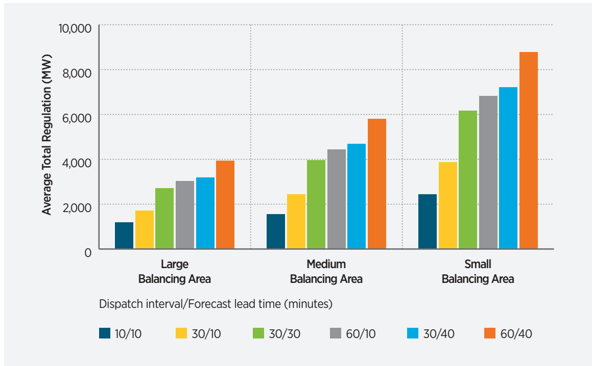
Figure 4-1. Increased balancing area size and faster scheduling reduce regulation requirements.
